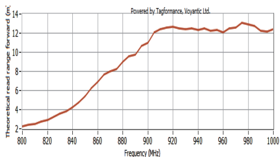
读距范围 (m) Read Range
