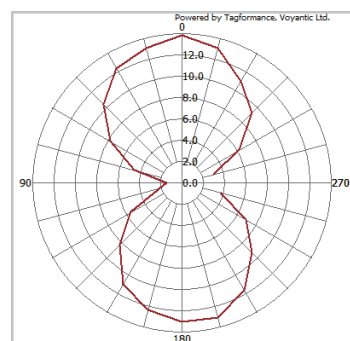
方位性 Orientation Sensitivity
