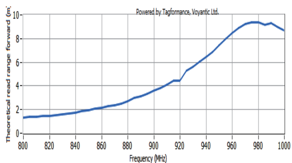
读距范围 (m) Read Range
